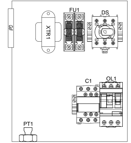
Standard Internal Layout
